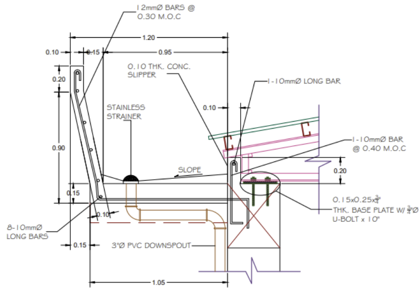
DETAIL OF CONC. GUTTER SCALE 1:20 MTS.
