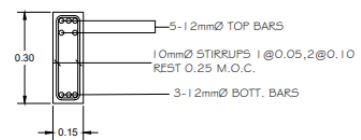
SECTION B-5
