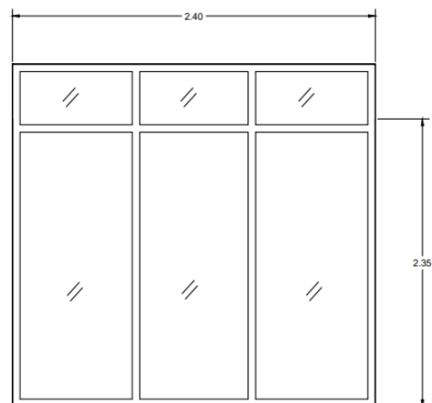
W2 SLIDING WINDOW W/ TRANSOM WINDOW 3 SETS
