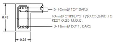
SECTION B-3
