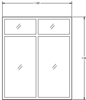
W4 SLIDING WINDOW W/ TRANSOM WINDOW 3 SETS
