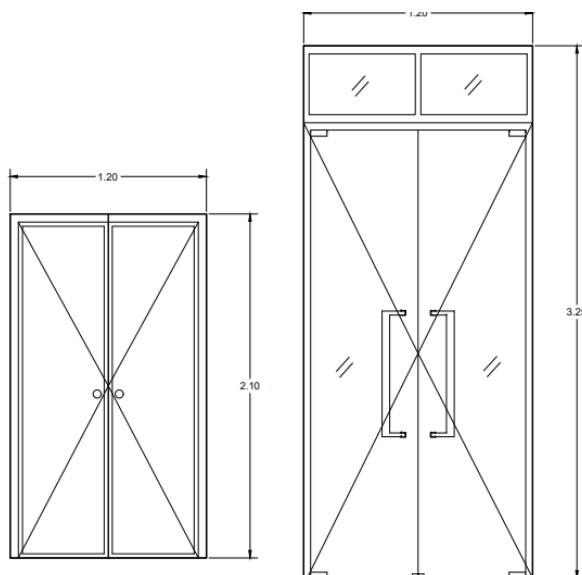
D2 FLUSH DOOR DOUBLE SWING TYPE 1 SET
