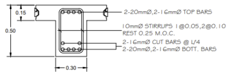
MIDSPAN B-1
