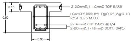
MIDSPAN B-2
