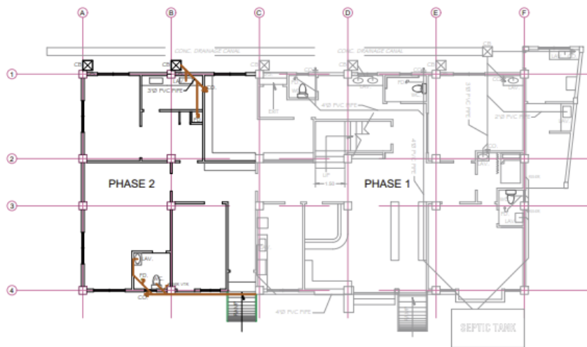
GROUND FLOOR PLUMBING PLAN SCALE 1:100 MTS.
