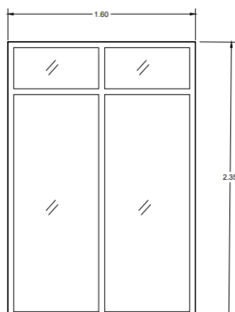
W1 SLIDING WINDOW W/ TRANSOM WINDOW 3 SETS
