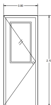
D5 SWING FLUSH DOOR W/ FIXED GLASS 2 SETS
