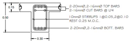
SUPPORT B-1
