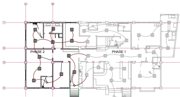
GROUND FLOOR LIGHTING LAYOUT SCALE 1:100 MTS.
