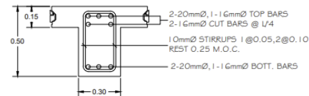
SUPPORT B-2
