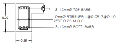
SECTION B-4
