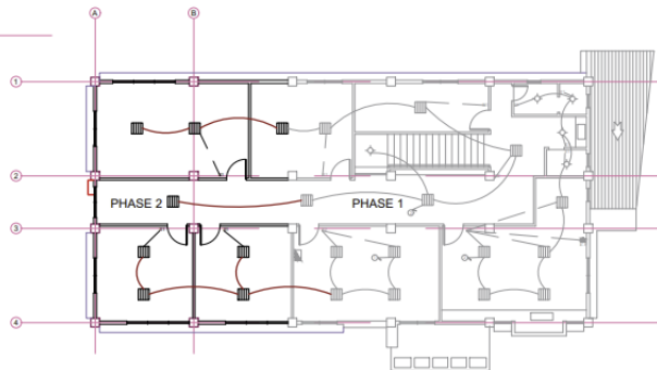
SECOND FLOOR LIGHTING LAYOUT
