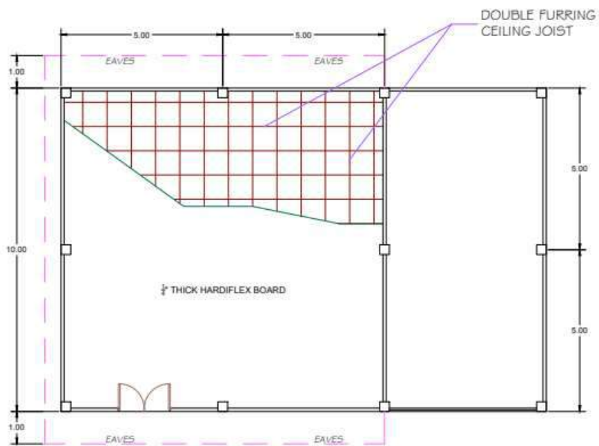
REFLECTED CEILING PLAN (w/ EXHAUST FAN)
